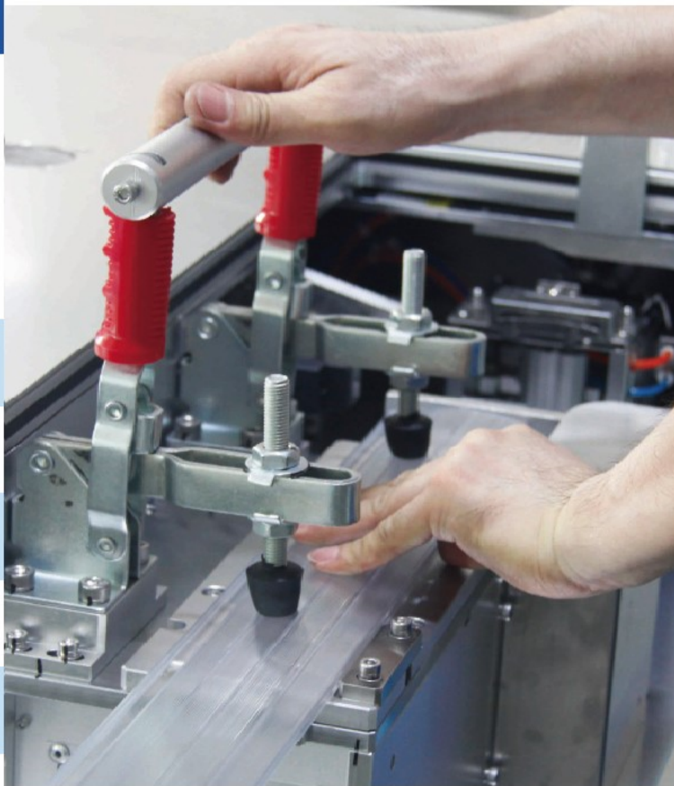
Automatic cover's slate technology 泳池电动盖浮条工艺
